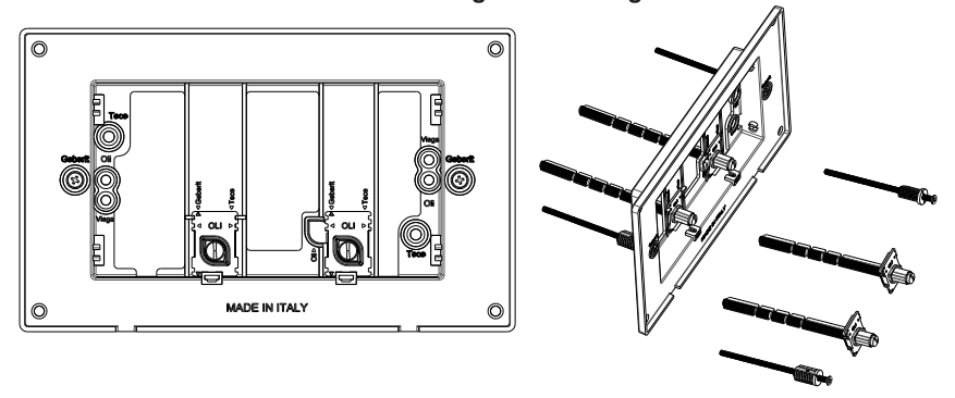
KIT102-Tece:2003-2020-2021-Now
